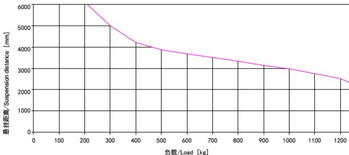
承载力数据图 A180 (仅供参考) / Load chart profile A180 (For reference only)
